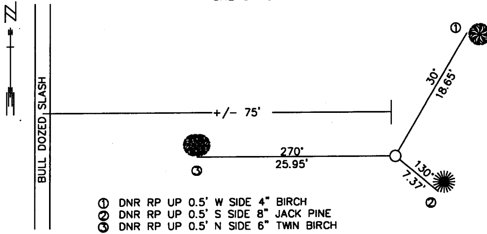
SKETCH OF REFERENCE TIES
