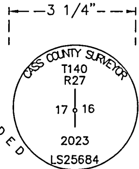
Cap Stamping Detail
