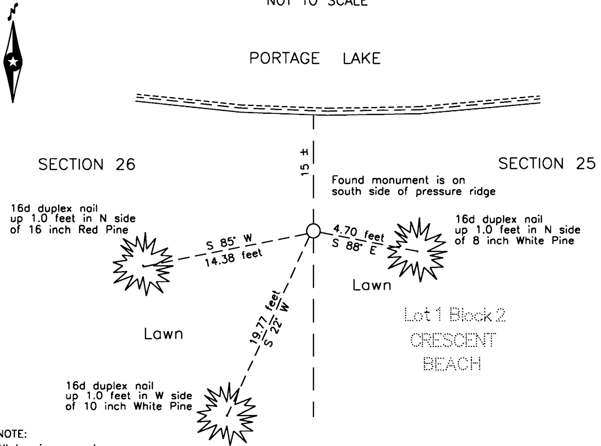
SKETCH OF REFERENCE TIES NOT TO SCALE
