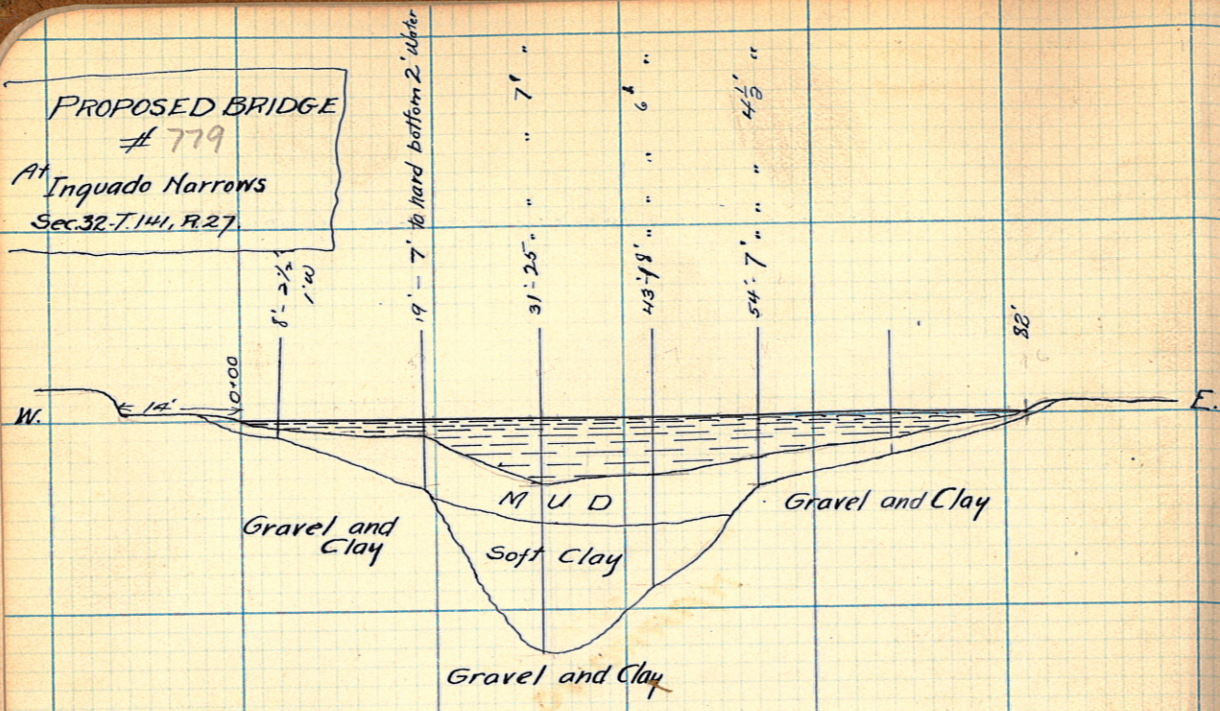
Cross Section of Narrows - Main Channel.
